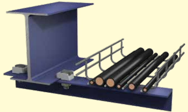
Cantilevered angle support for running cable tray
